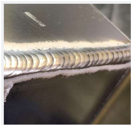
An example of a strong and visually pleasing aluminium TIG weld
